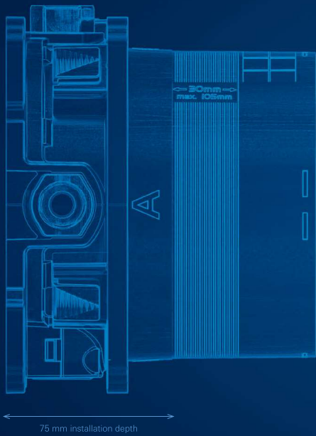
75 mm installation depth
